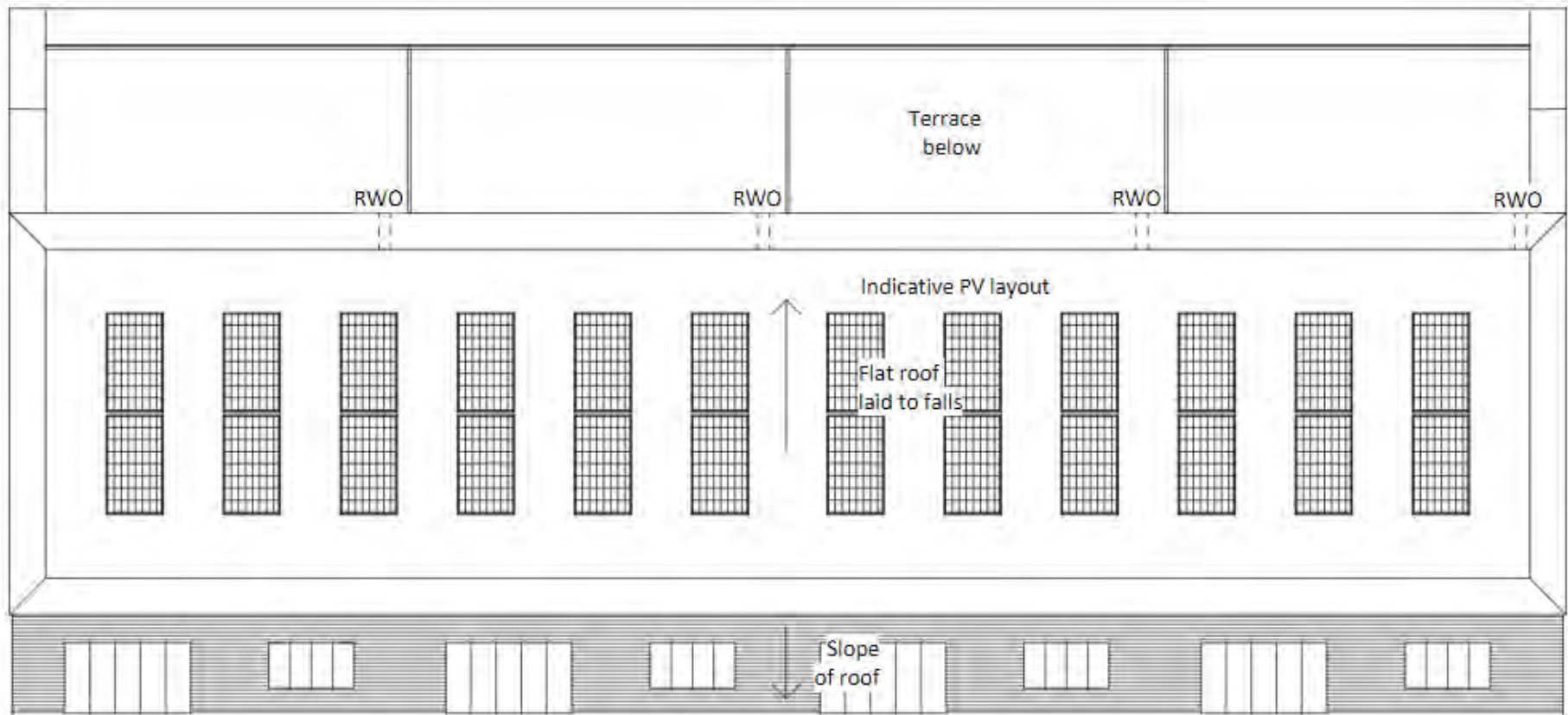
Figure 14 - Block H and J Roof Layout
